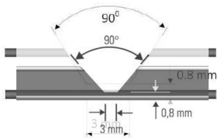
V-shaped 90° Groove
