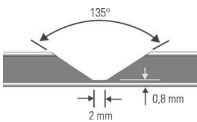
V-shaped 135° Groove
