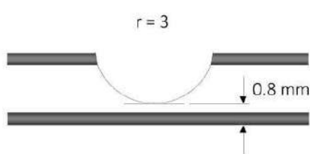
Circular Groove
