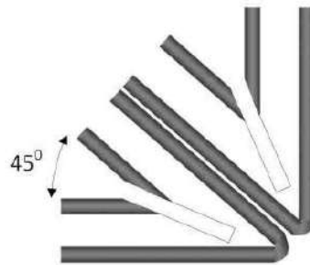
V-shaped 135° Groove if folded up to 45°
